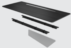
DESK TOP frame support & hardware + reversible Blanco Laminate Modesty panel and mounting brackets (2)
